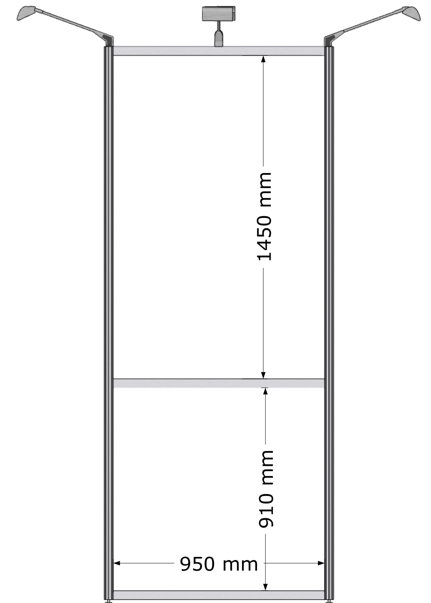
TYPICAL ELEVATION
